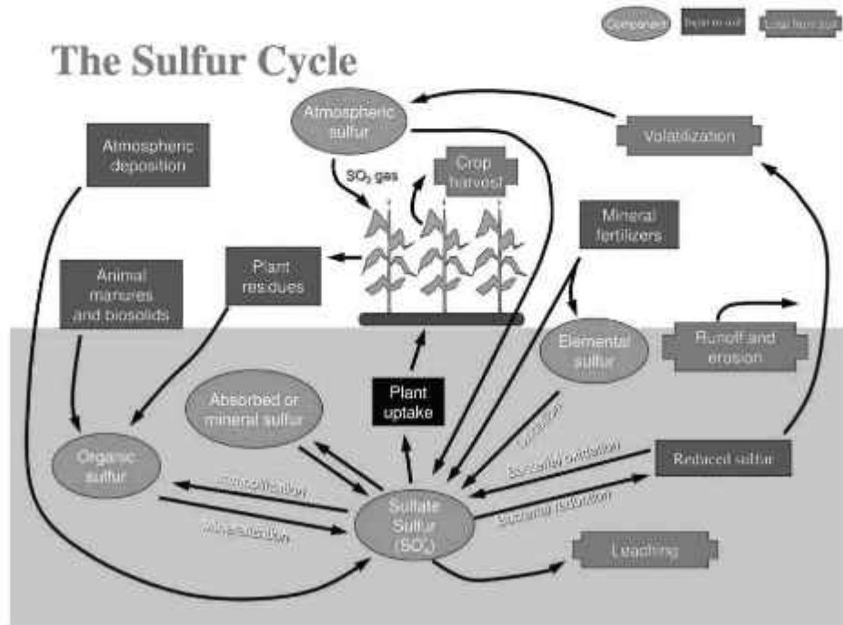
Photograph 1.12: Sulphur Cycle
