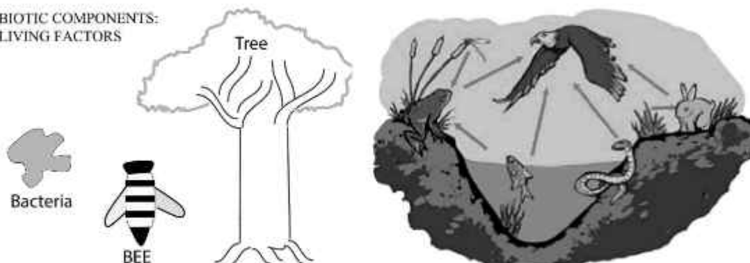
Photograph 1.6: Biotic Components
