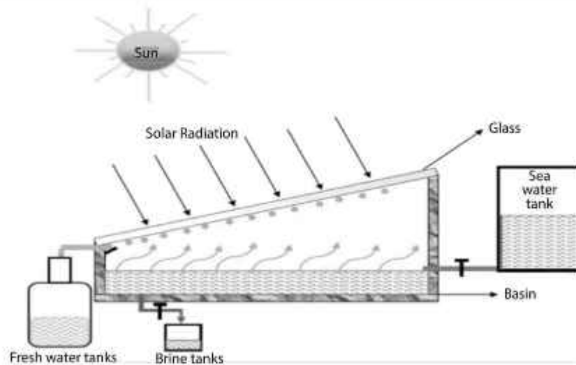
Photograph 3.5: Solar Stills
