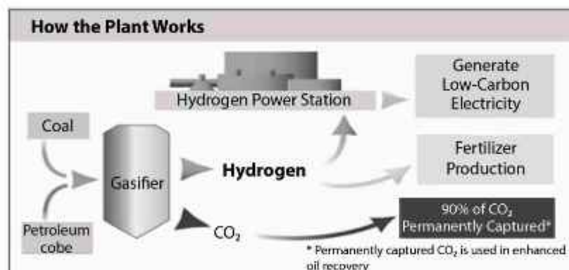
Photograph 3.10: Hydrogen Energy
