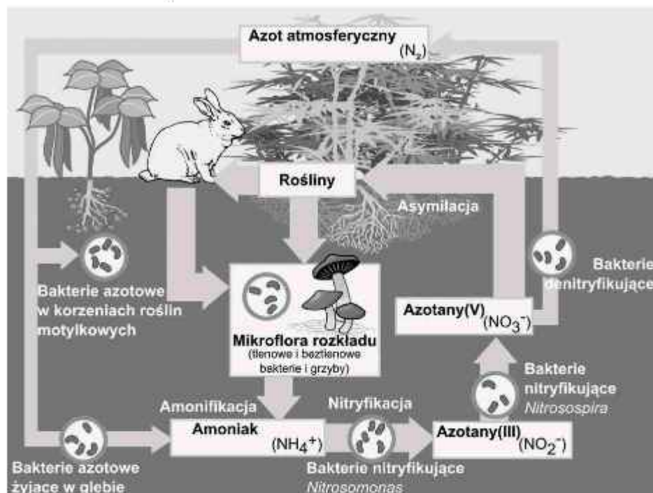
Photograph 1.11: Nitrogen Cycle
