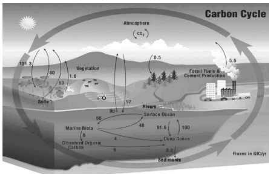
Photograph 1.10: Carbon Cycle
