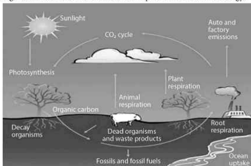
Photograph 1.1: Ecosystem
