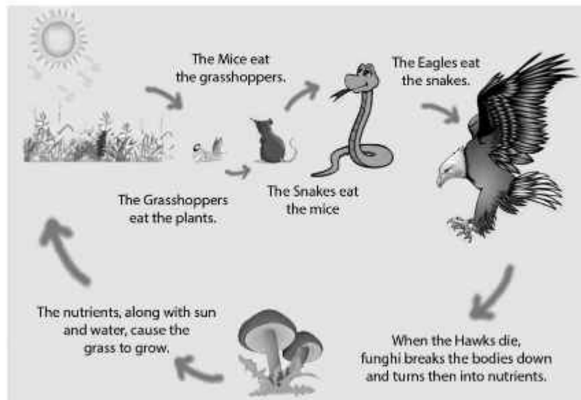
Photograph 1.8: Food Chain
