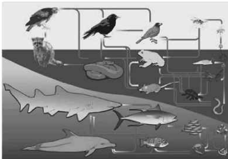
Photograph 1.9: Food Web
