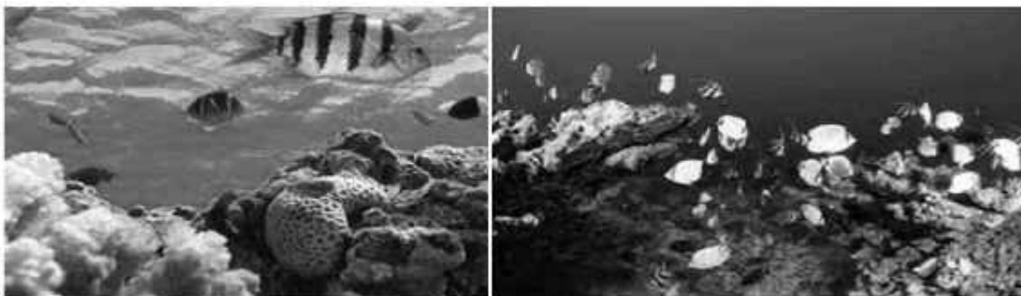
Photograph 1.3: Aquatic Ecosystem
