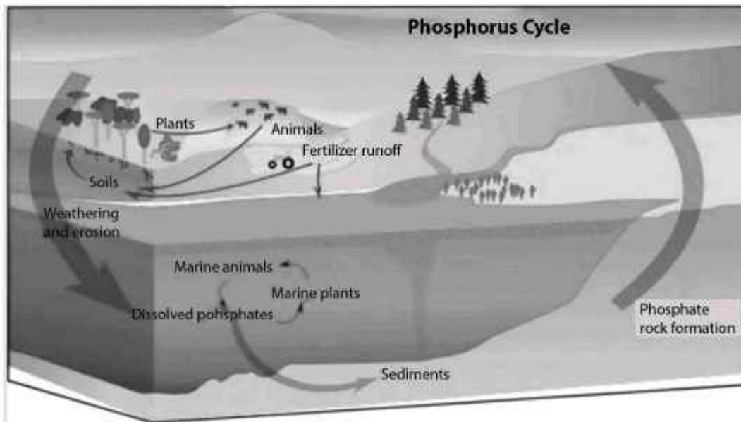
Photograph 1.13: Phosphorus Cycle
